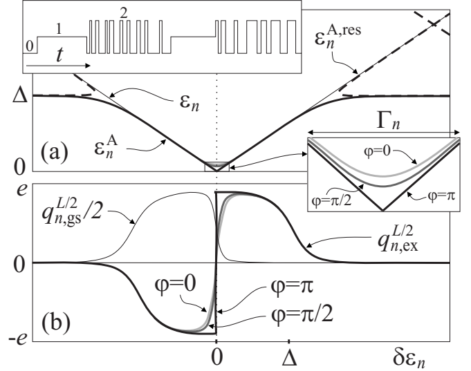
FIG. 2. (a) Bound state \varepsilon_n^A (thick solid lines) and resonances \varepsilon_n^{A,res} (dashed lines) in the Andreev dot versus position \delta\varepsilon_n of the normal-state resonance (tuned via the gate potential V_g ); we choose \Gamma_n = 0.2\Delta . Also shown are the normal resonances \varepsilon_n (thin solid line) and the dependence on the phase difference \varphi across the dot (inset). (b) Charges q_{n,gs}^{L/2} and q_{n,ex}^{L/2} . Top inset: structure of telegraph noise with long periods of ground state (0) and singly occupied (1) states and the ground-state trace interrupted by fast doubly excited states (2).
