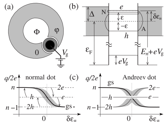
FIG. 1. (a) Andreev dot (SINIS) embedded in a superconducting ring. Tuning of flux \Phi or gate potential V_g serves to modify the charge on the dot. (b) The mixing of Andreev and normal scattering at a SIN boundary leads to particle-hole symmetry breaking and to the appearance of a fractional charge on the dot. The phenomenon shows up in the vicinity of a resonance in the associated NININ device, here, an electron-type resonance, where the electron quasi-particle is multiply reflected while the hole component is not. (c) Charge trapped on normal and Andreev dots versus position of resonance \delta\varepsilon_n ; shown are the ground-state (gs) and single-particle excited-state charges for the singly and doubly occupied situation. gs: as the resonance passes the Fermi level, a charge of 2e is pushed out of the dot over a width \Gamma_n ; the shaded areas indicate the importance of quantum fluctuations. Dashed lines (normal dot) indicate electron- and hole-type resonances; the associated trapped charges decay rapidly to the ground-state charge (arrows). These resonances are transformed into eigenstates in the Andreev dot; they carry integer charge if occupied once (odd parity) and a fractional charge when occupied twice (even parity).
