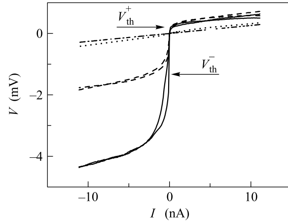
Fig.3. I - V curves for total filling factor \nu = 2 and g = 1 under the gate at different tilt angles. They are: \theta = 0^\circ (solid line), \theta = 30^\circ (dashed line), \theta = 45^\circ (dotted line). Dash-dot line depicts fully equilibrium I - V curve, calculated from Landau-Buttiker formulas. The normal magnetic field is constant and equals to 8.7 T
