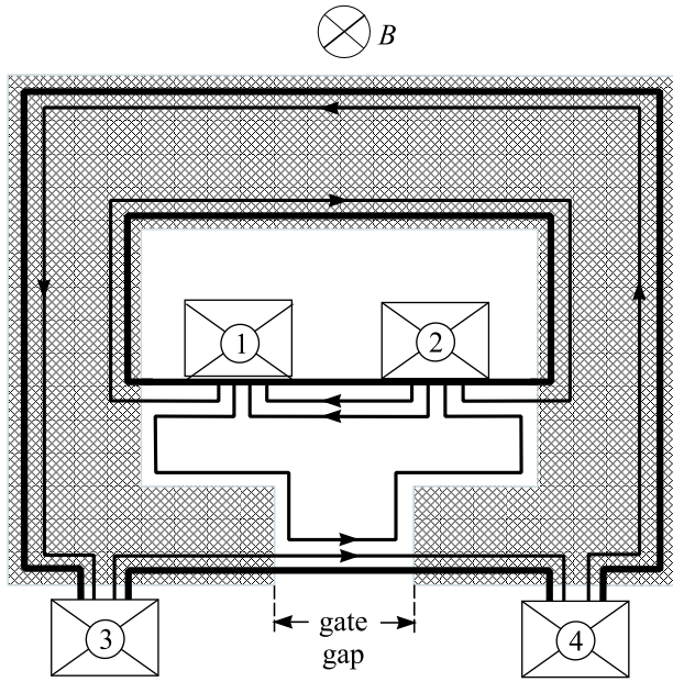
Fig.2. Schematic diagram of the pseudo-Corbino geometry. Contacts are positioned along the etched edges of the ring-shaped mesa (thick outline). The shaded area represents the Schottky-gate. Arrows indicate the direction of electron drift in the edge channels for the filling factors \nu = 2 in the ungated regions and g = 1 under the gate
