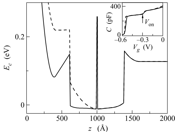
Fig.1. Quantum well subband diagram at zero gate voltage (solid line) and at twice smaller electron concentration (dashed line) as calculated from the growth sequence of the structure (calculated using Poisson–Schrodinger solver by G. Snider). Inset shows the capacitance of the sample in dependence on the gate voltage calculated from the subband diagram (dashed) and measured in the experiment (solid). The magnetic field is zero
