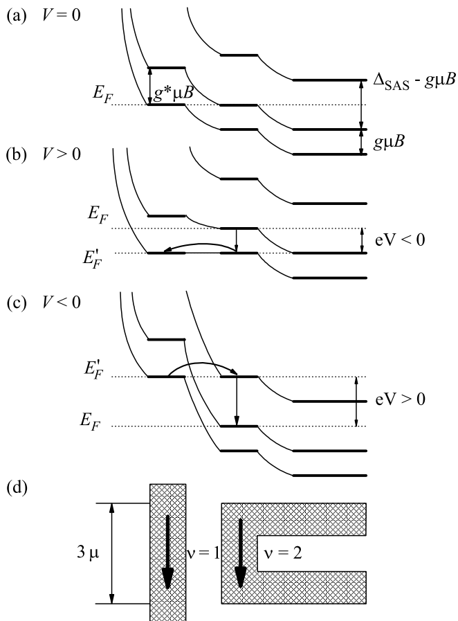
Fig. 5. Energy subband diagram of the sample edge in the gate-gap for the filling factors \nu = 2 and g = 1 . (a) No voltage V applied between the inner and outer ES. (b) V > 0 , in the situation shown, the outer ES is shifted down in energy by eV = -|g|\mu_B B . (c) V < 0 , here the energy shift eV > 0 . (d) Sketch of the compressible strips in the gate-gap region. Arrows in Figs. 5b and 5c indicate new ways for electron relaxation opening up at high potential imbalance
